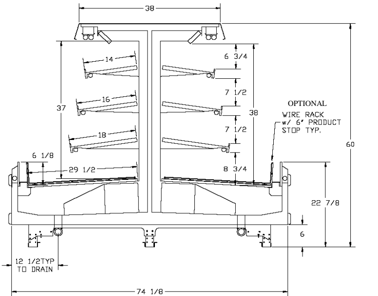
CENTER ISLAND CROSS-SECTION
