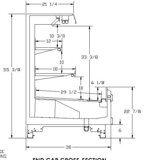
END CAP CROSS-SECTION
