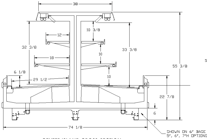
CENTER ISLAND CROSS-SECTION
