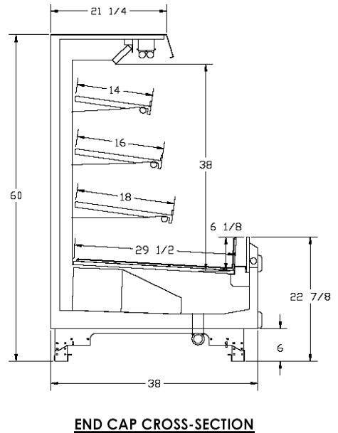
END CAP CROSS-SECTION
