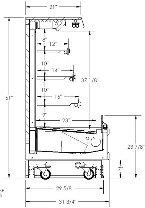
END CAP CROSS-SECTION
