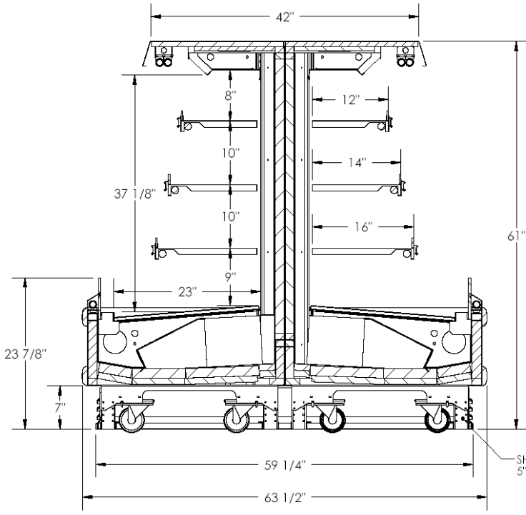
CENTER ISLAND CROSS-SECTION
