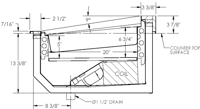
SSB-6-DI "DROP-IN" CONVERTIBLE SALAD BAR (SHOWN WITH SALAD PANS REMOVED)
