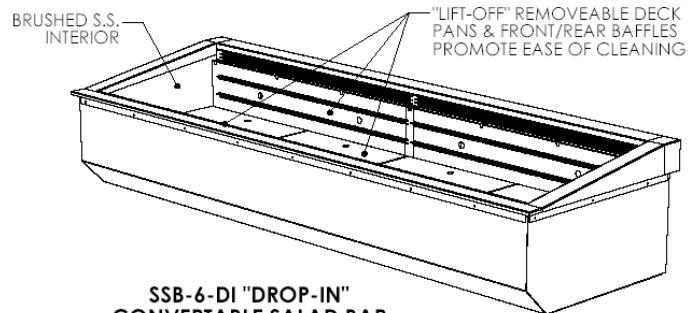
SSB-6-DI "DROP-IN" CONVERTIBLE SALAD BAR (SHOWN WITH SALAD PANS)
