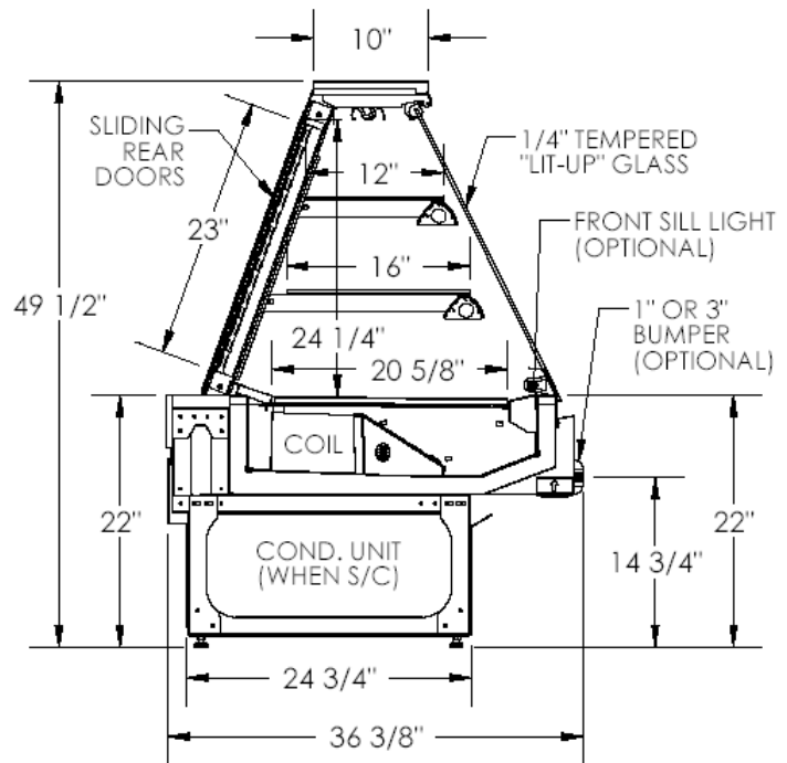
SFBIF - FLAT GLASS FRONT SERVICE BAKERY CASE
