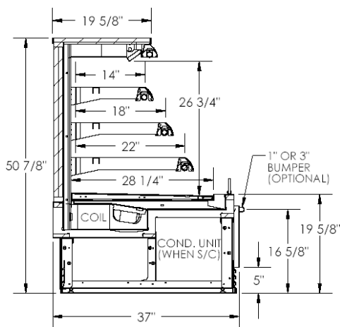
SFBO - OPEN FRONT SELF SERVICE BAKERY CASE
