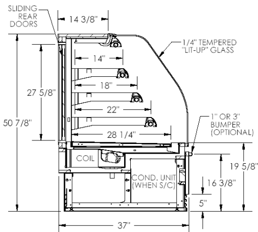
SFB - CURVED GLASS FRONT SERVICE BAKERY CASE
